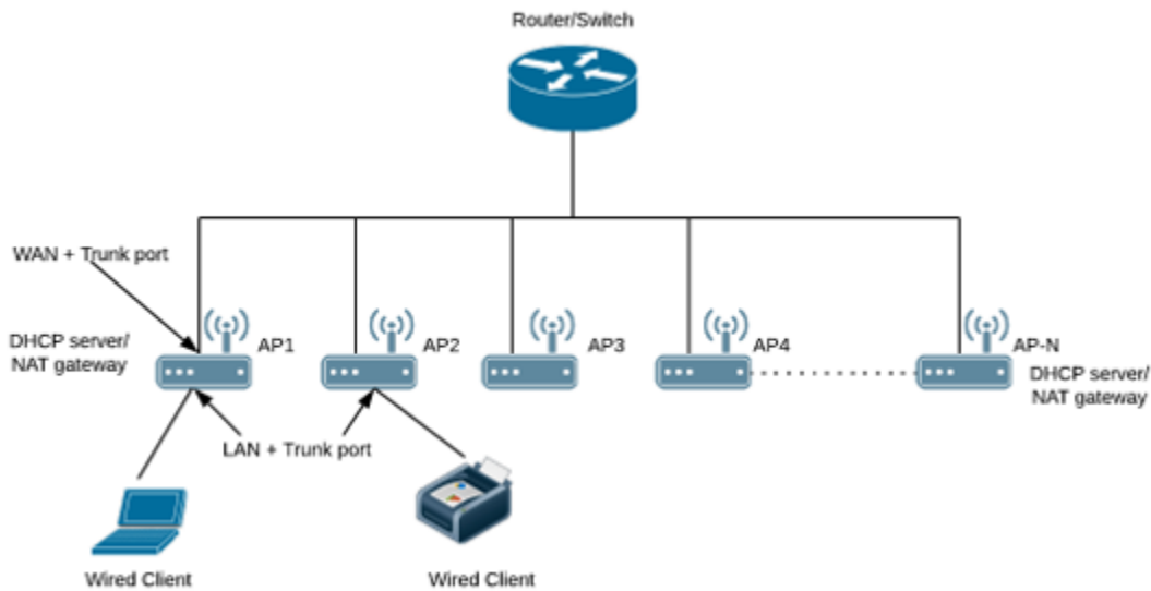
FIGURE 201 Single AP Topology
