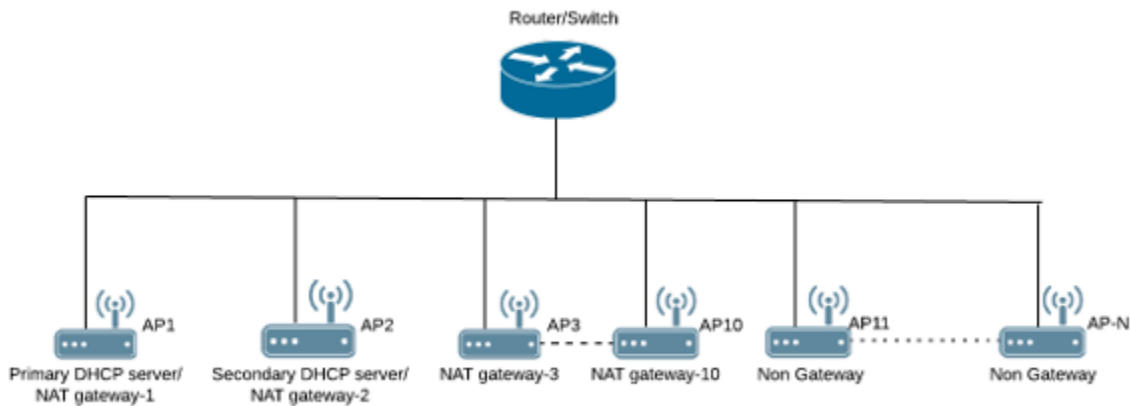
FIGURE 202 Multiple AP (Flat Network) Topology
