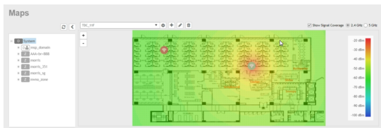
FIGURE 34 RF Coverage Heat Map
