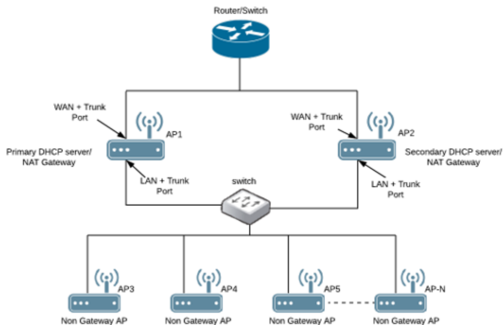
FIGURE 203 Hierarchical AP Topology
