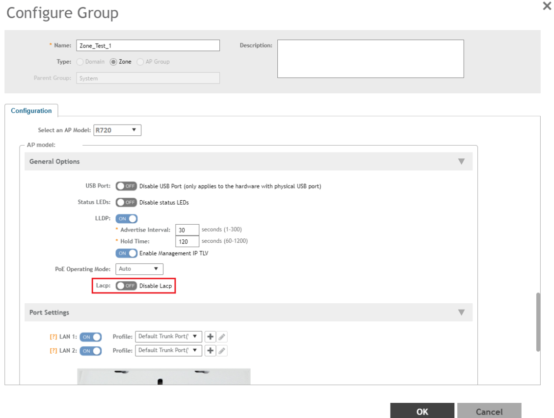
FIGURE 53 Enabling LACP Support for a Zone
