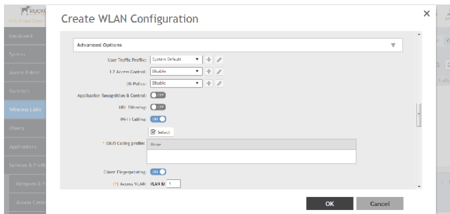
FIGURE 179 Configuring WiFi Calling in a WLAN
