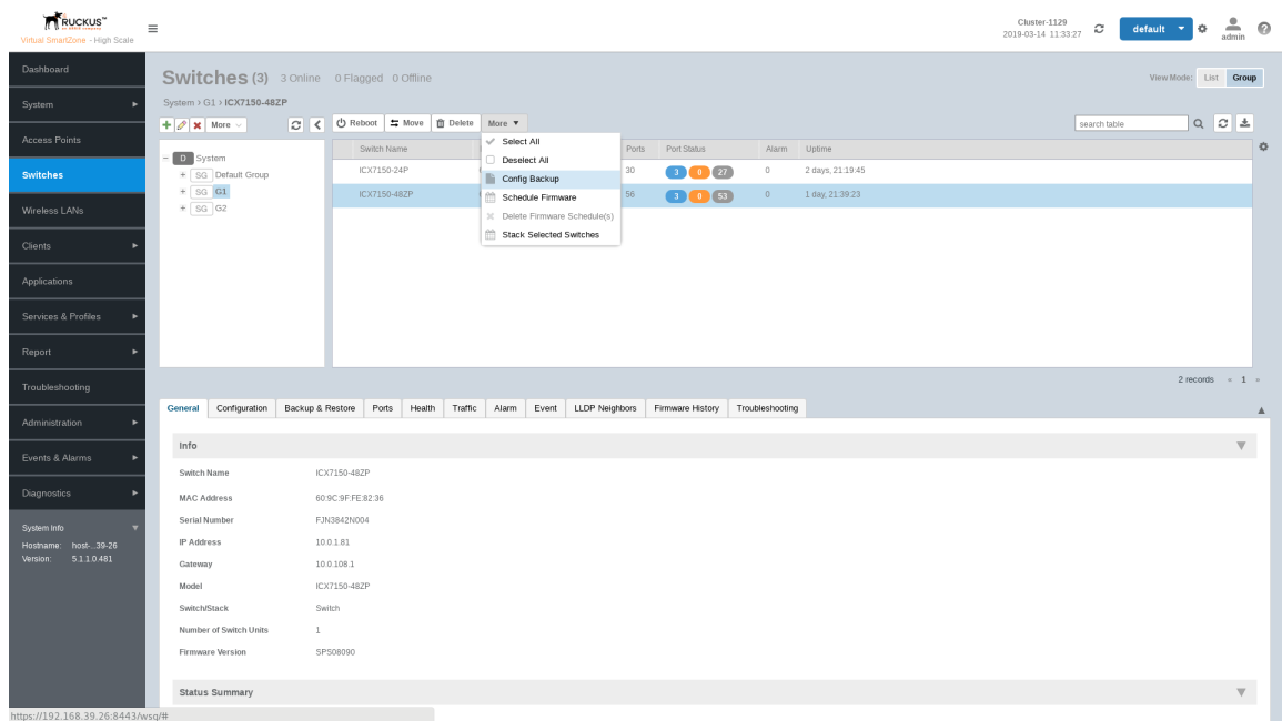
FIGURE 68 Configuring Backup
