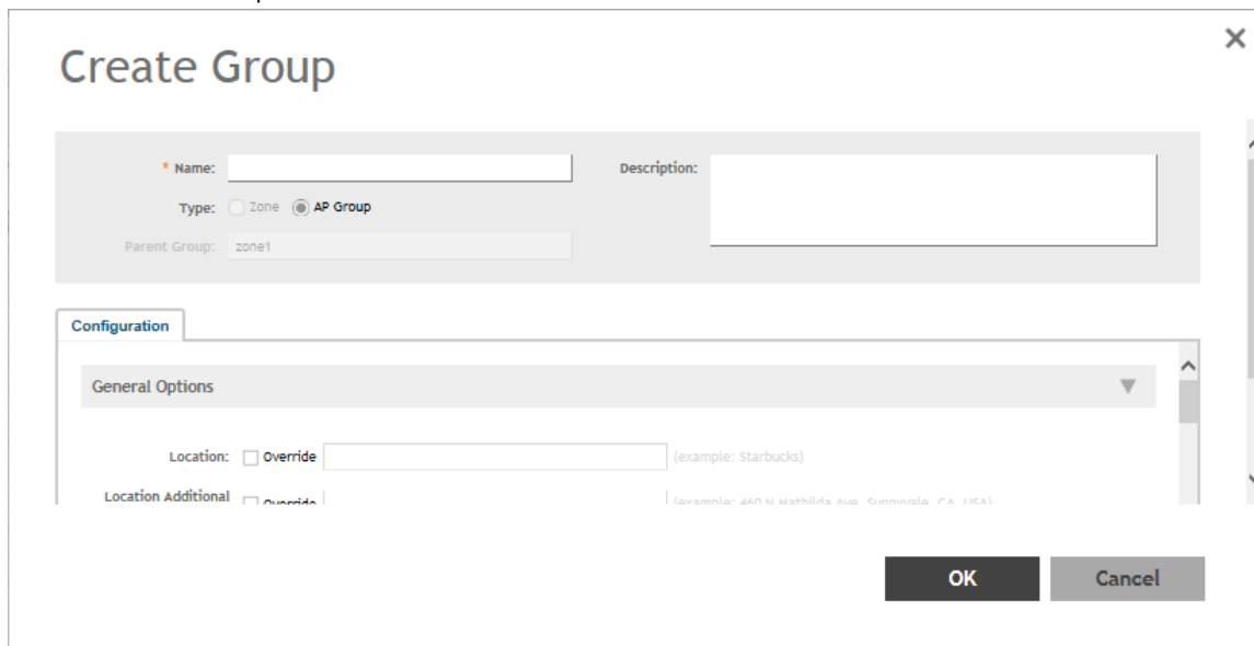
FIGURE 42 Create Groups
