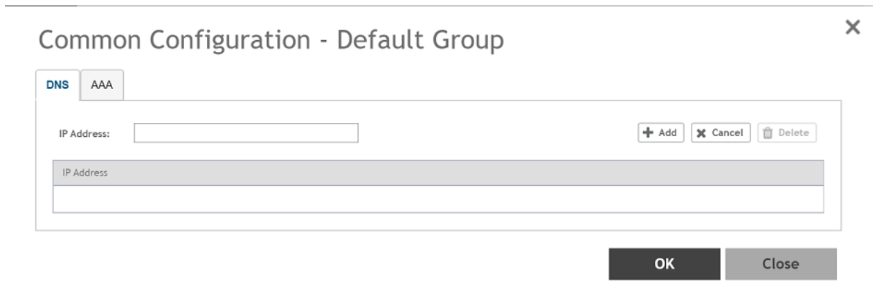
FIGURE 73 DNS Settings
