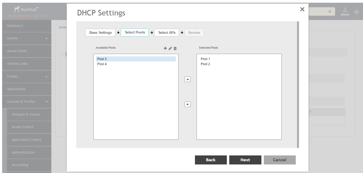
FIGURE 206 Selecting Pools
