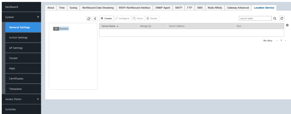
FIGURE 27 Location Service
